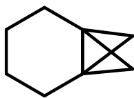
[4.1.1]propellane
