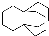
[4.4.4]propellane
