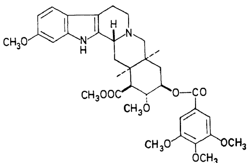
Reserpine
