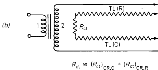
Figure 4. Coupled charge transfer reactions, O + e^- \rightleftharpoons OR , OR + e^- \rightleftharpoons R : (a) general form of circuit; (b) circuit for C_{OR} \ll C_O , C_{OR} \ll C_R when R_{ct} is small
