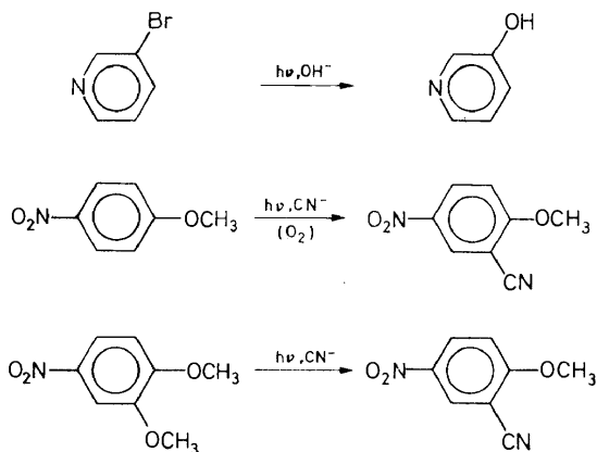
Figure 5. Photohydrolysis of 3-bromopyridine 2h ; photocyanation 4
