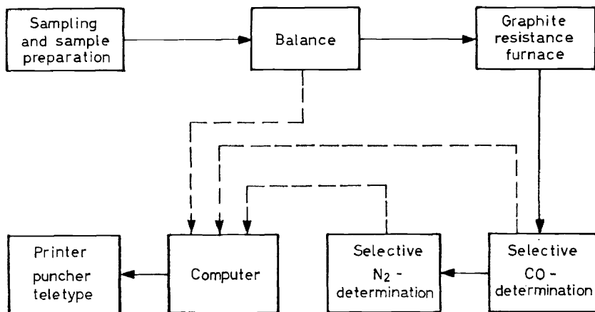
Figure 8. Scheme of an automatic equipment for determining nitrogen and oxygen
