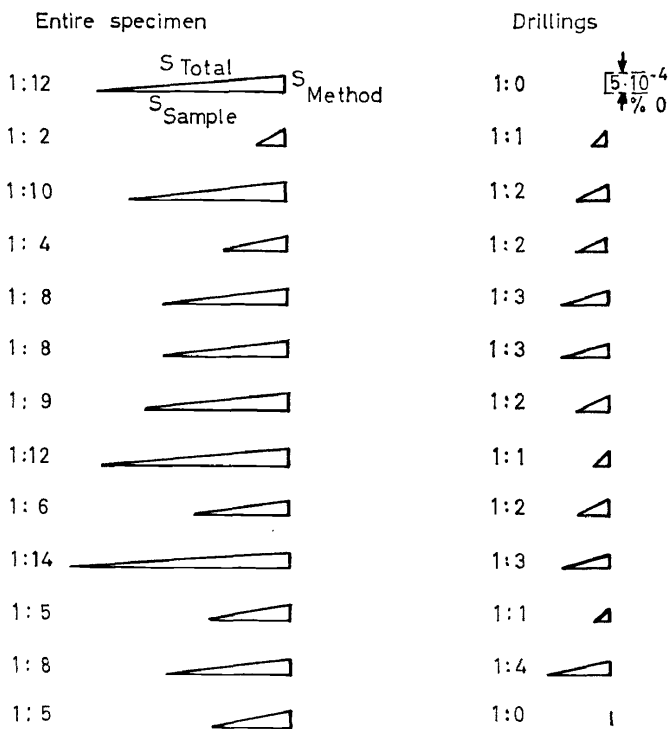
Figure 9. Oxygen determination: comparative investigations
