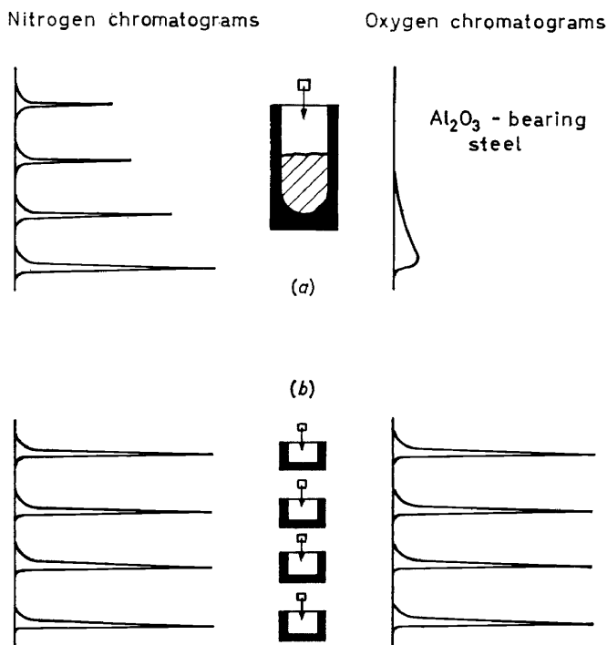
Figure 12. Degassing curves: (a) Large crucible with metal bath; (b) Small crucible without metal bath
