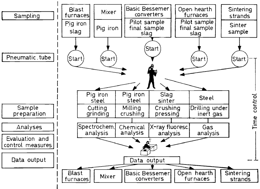
Figure 6. Scheme of sample preparation laboratory
