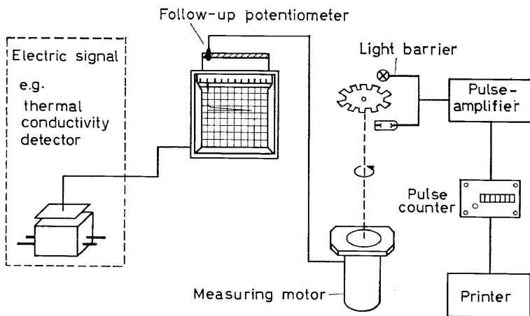
Figure 3. Conversion of non-integrated analogue signal into digital reading
