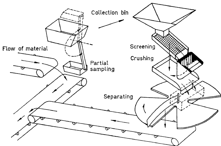
Figure 4. Automatic ore sampling
