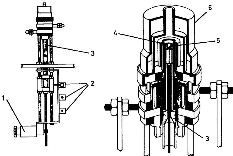
Figure 13. Furnace design and replacing of crucible (1, Motor for crucible elevator; 2, Controlling contacts; 3, Crucible elevator; 4, Heating element; 5, Graphite crucible; 6, Cooling jacket)
