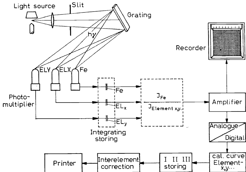
Figure 2. Conversion of integrated electric valve into digital reading
