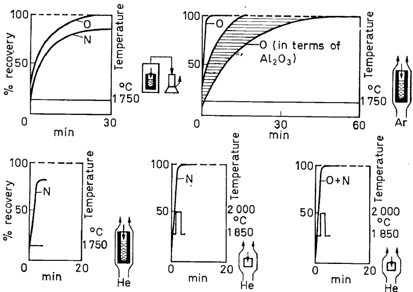
Figure 11. Effect of temperature control, crucible size and charge on the evolution of gas
