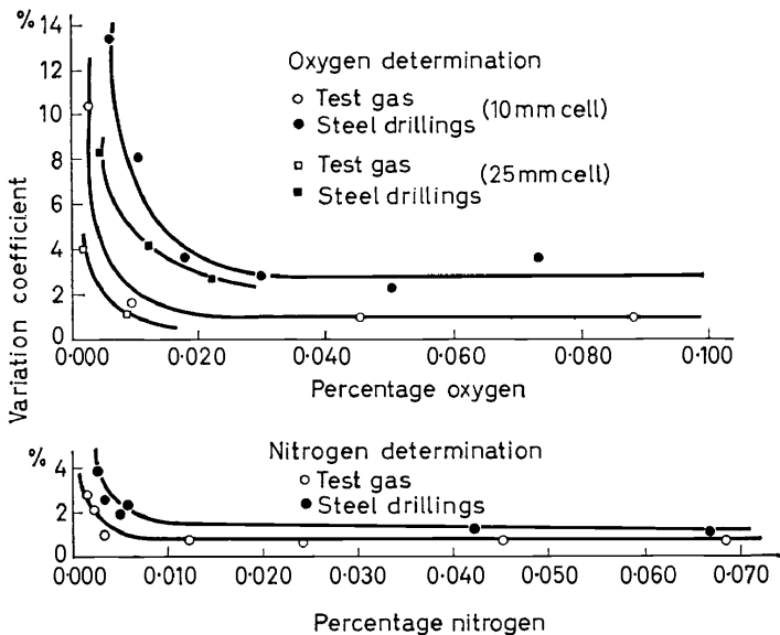
Figure 15. Variation coefficient as a function of content
