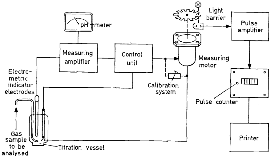
Figure 1. Principle of pulse coulometry
