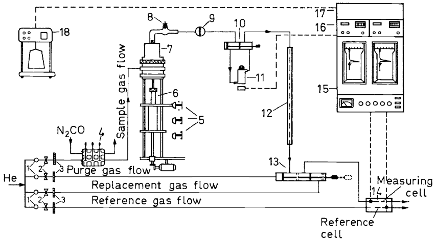
Figure 14. Scheme of instrument for combined determination of nitrogen and oxygen (1 Constant pressure regulator; 2, Precision regulating valve; 3, Flow meter; 4, Calibrating valve; 5, Limit switch; 6, Crucible elevator; 7, Graphite resistance furnace; 8, Sample port; 9, Dust filter; 10, Valve; 11, Cell; 12, Separation column; 13, Magnetic valve; 14, Thermal conductivity detector; 15, Recorder; 16, Integrator; 17, Computer; 18, Balance
