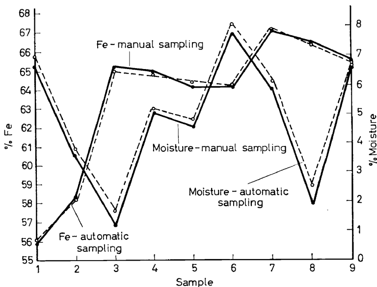
Figure 5. Comparison of automatic and manual sampling
