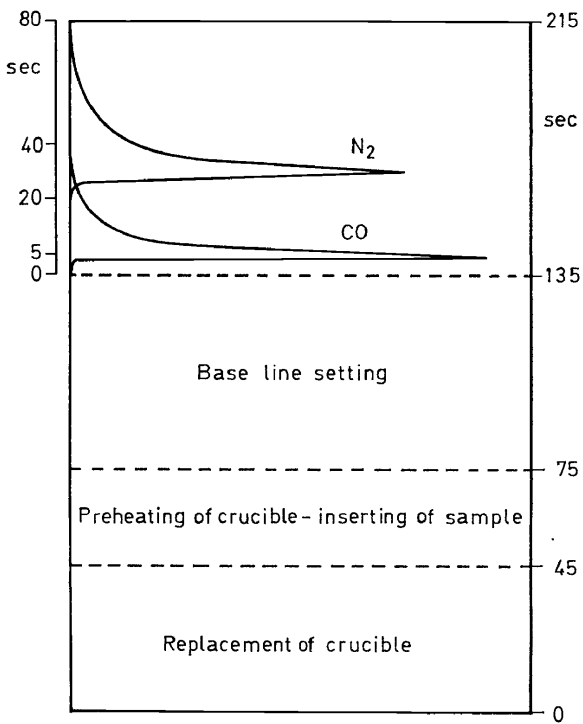
Figure 16. Time required for combined determination of nitrogen and oxygen
