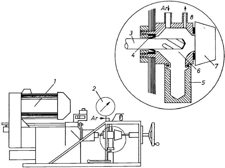
Figure 10. Device for making drillings under argon (1, Hydraulic horizontal drilling machine; 2, Pressure gauge; 3, Drilling bit; 4, Shaft gasket; 5, Copper vessel; 6, Drilling chamber; 7, Sample; 8, Lead sealing)
