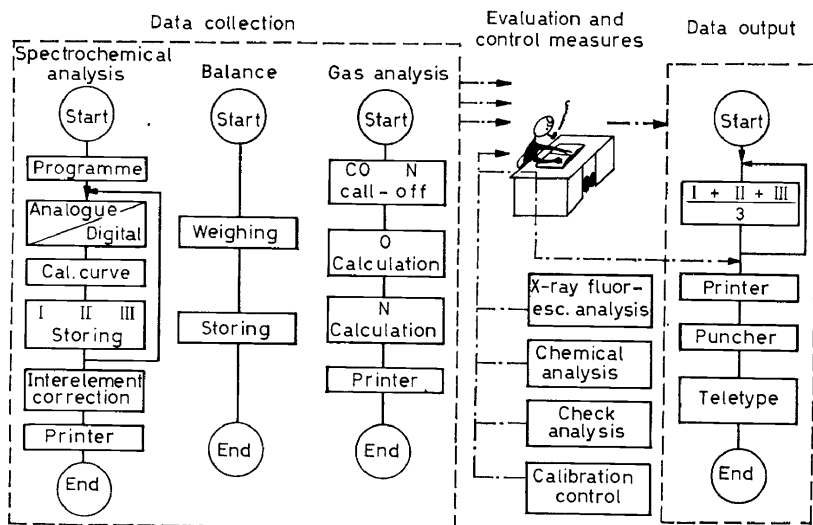
Figure 7. Scheme of automatic analysis cycle
