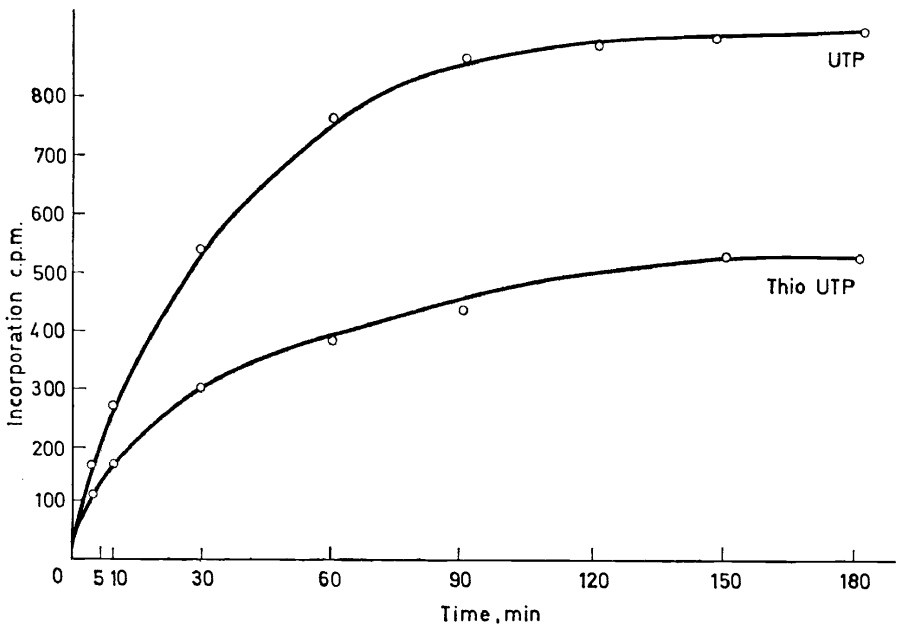
Figure 29. Incorporation of thio UTP with RNA-polymerase (50 nmole ATP- 14 C, 50 nmole thio UTP, 0.1 O.D. poly dAT) [K.-H. Scheit, H. Matzura, F. Cramer, Göttingen 1967]
