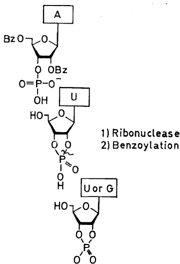
Figure 27. Synthesis of a ribotrینucleotide [W. Siehr, F. Cramer, Göttingen 1966]
