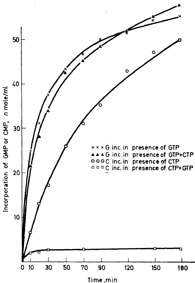
Figure 7. Incorporation of GMP and CMP; template: poly dGdC [H. Matzura, Göttingen 1967]
