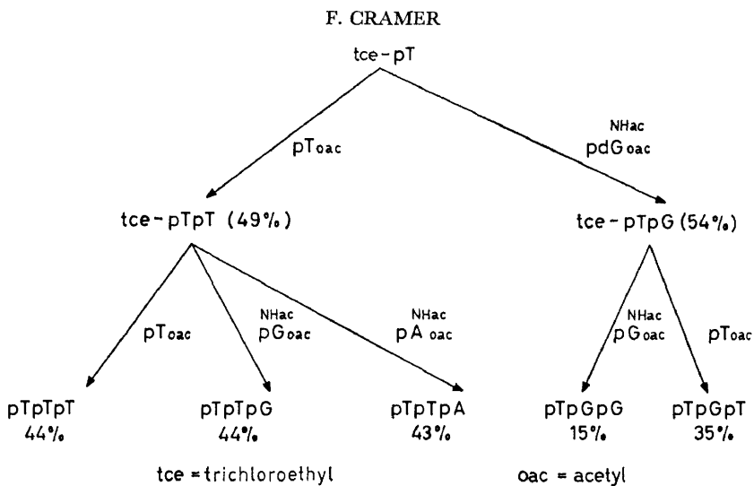
Figure 14. Stepwise synthesis of trinucleotides using trichloroethyl protecting group [A. Franke, K.-H. Scheit, F. Eckstein, Göttingen 1966]
