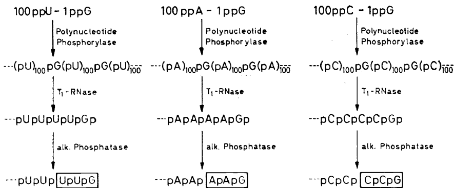
Figure 32. Synthesis of ribopolynucleotides with defined 3'-terminal triplet by cleavage with T 1 -ribonuclease [H. Küntzel, Göttingen 1964]
