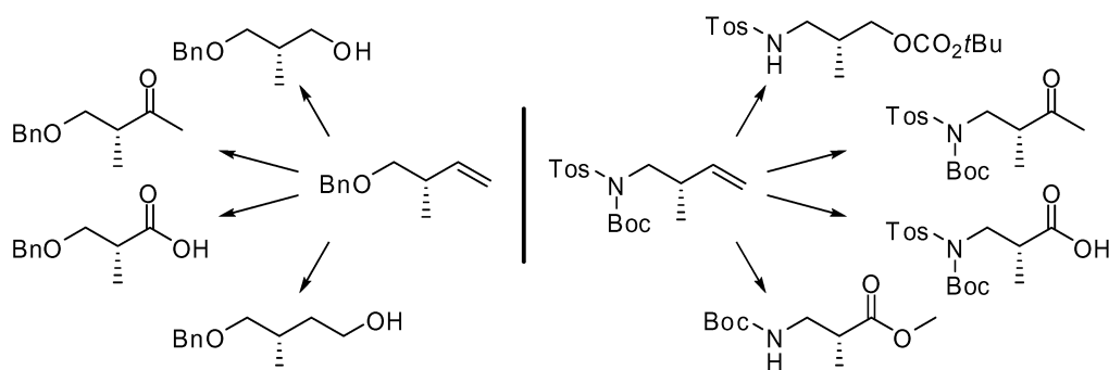
Fig. 2 Multifunctional building blocks from AAA products.
